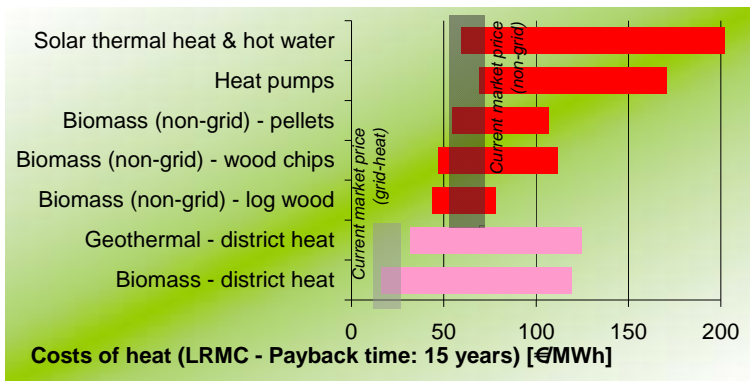
Figure III-4. Long-run marginal generation costs for the year 2010 for various RES-H options in EU countries (Green-X 2011)
