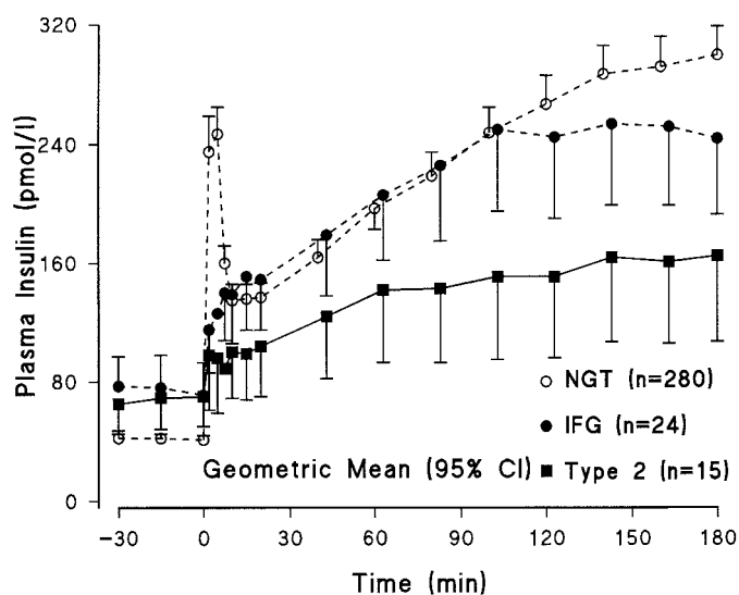
FIG. 1. Geometric mean (95% CI) plasma insulin levels during 180-min hyperglycemic glucose clamps (10 mmol/l) in 280 NGT subjects, 24 IFG subjects, and 15 type 2 diabetic subjects.
