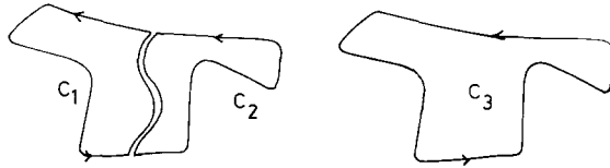
Fig. 3. If C_1 and C_2 together span the same area as the single curve C_3 the restrictions A(C_1)A(C_2) = A(C_3) and B(C_1)B(C_2) = B(C_3) are consistent with the commutation rules although the first do not follow from the definition of A .
